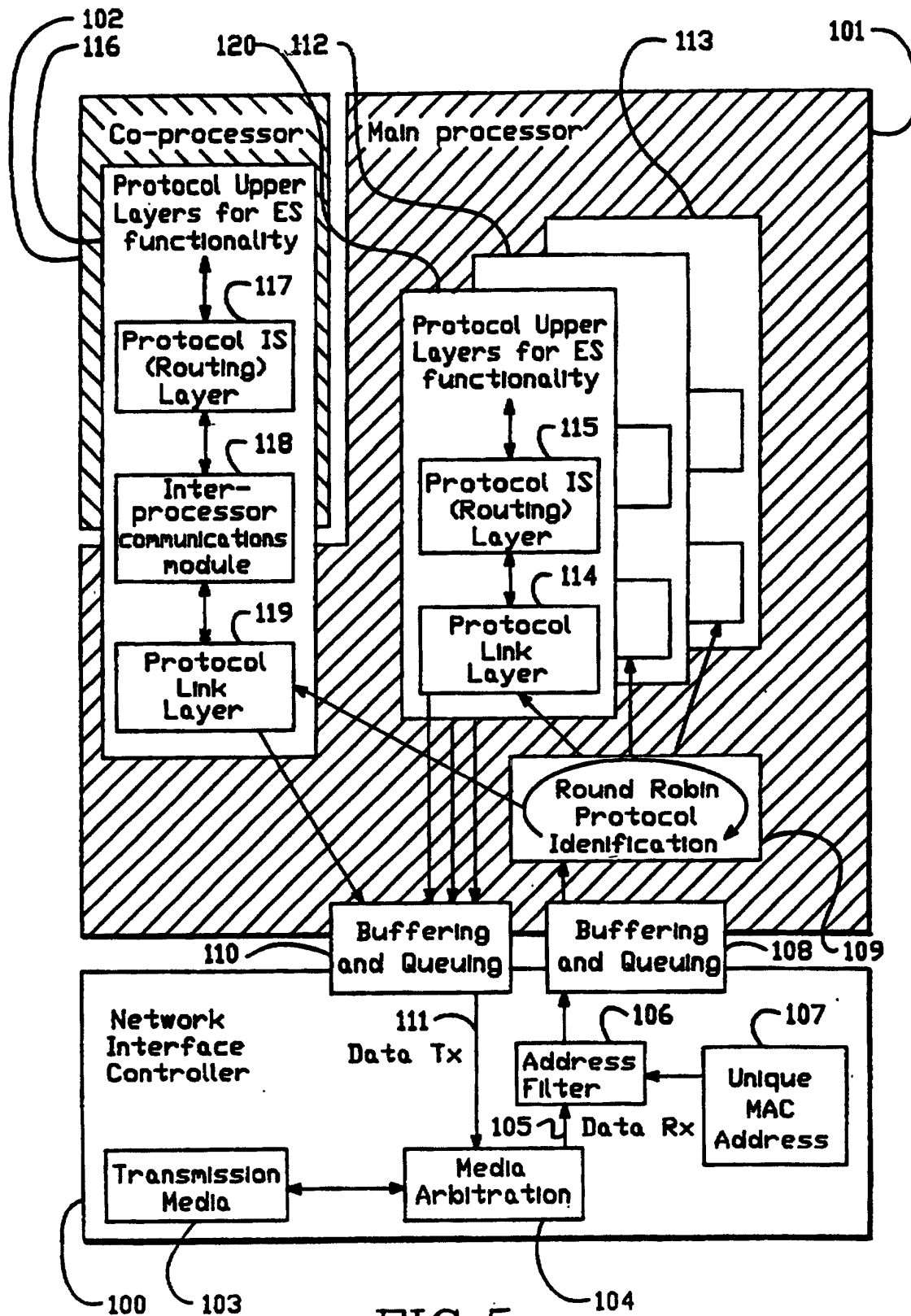
FIG. 5 (PRIOR ART)
