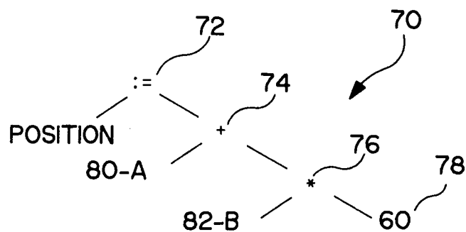
SYNTAX TREE FOR "POSITION:= A + B * 60"
