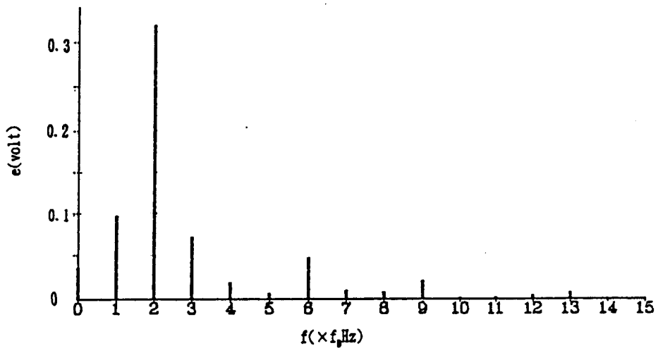
(b) Skipped M-sequence e_{SM}
