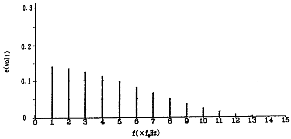
(a) M-sequence e_M
