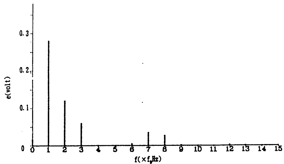
(c) Shaped M-sequence e_{SS}
