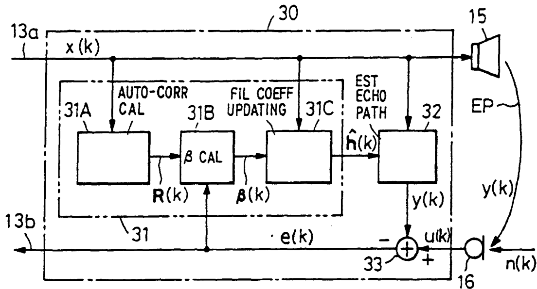
FIG. 5 PRIOR ART
