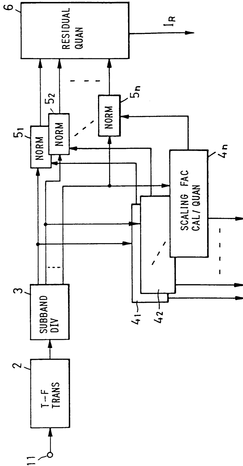
FIG. 1 PRIOR ART
