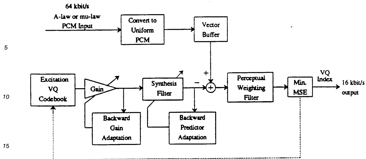
LD-CELP Encoder
