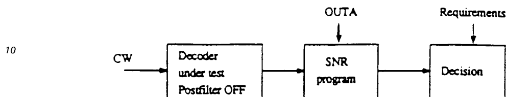
FIGURE I-2/G.728
