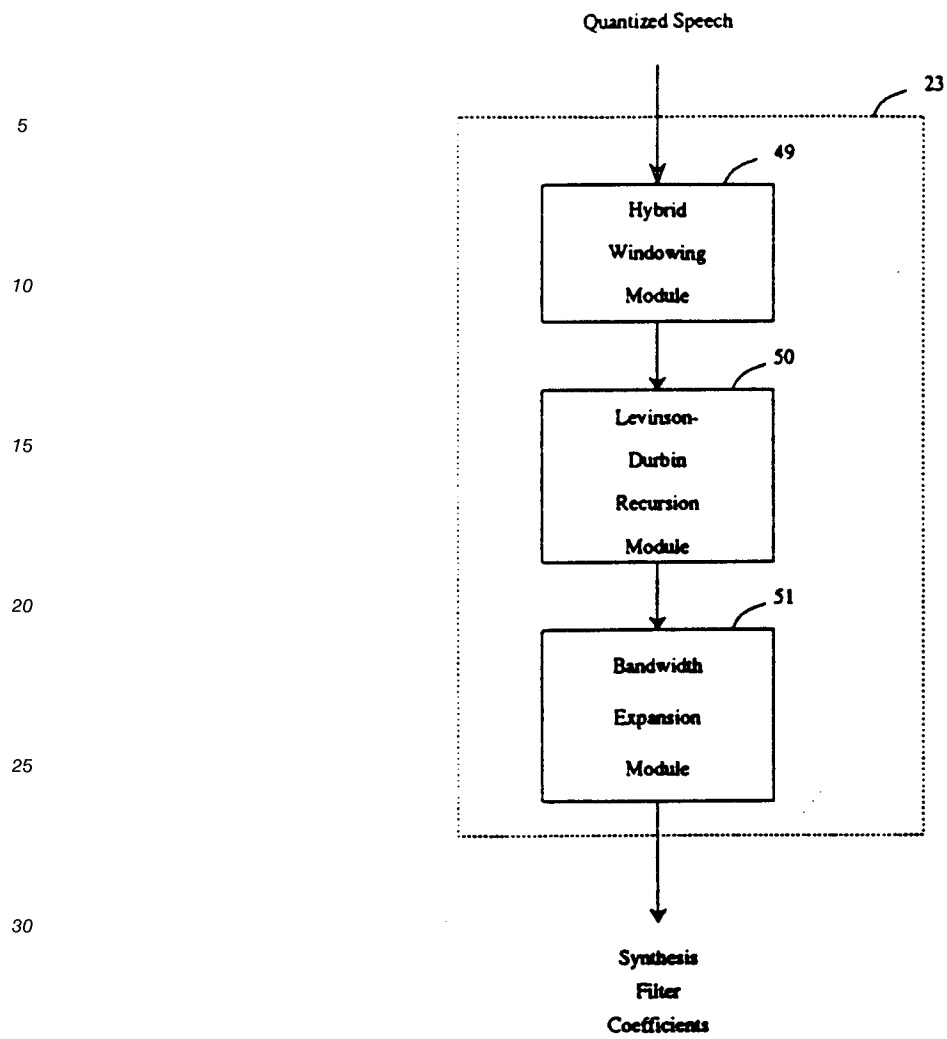
Figure 5/G.728 Backward Synthesis Filter Adapter
