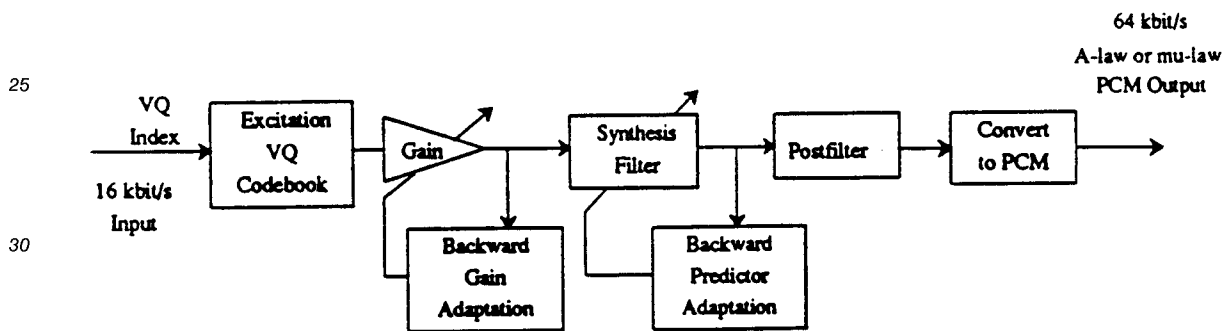
LD-CELP Decoder
