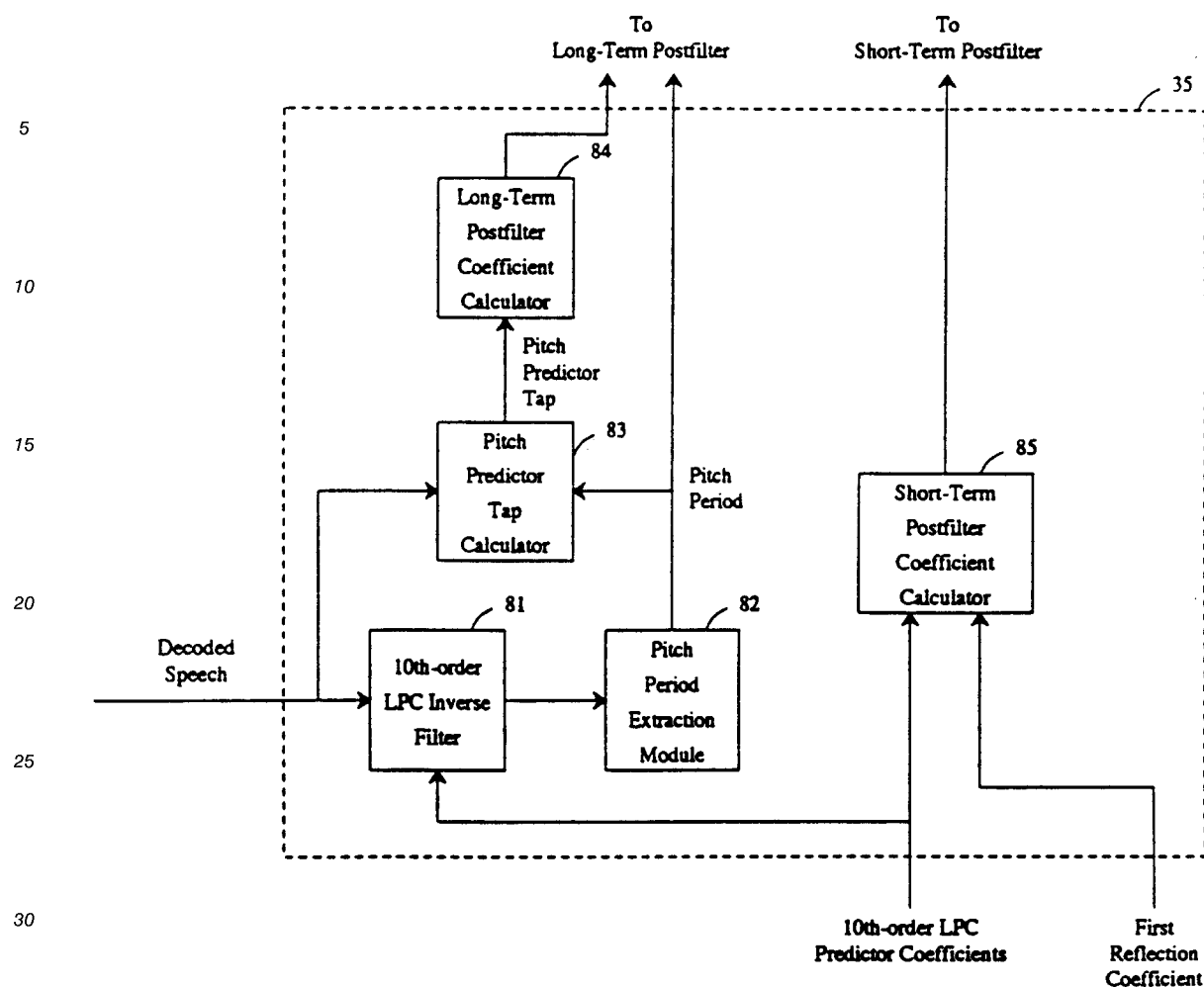
Figure 8/G.728 Postfilter Adapter Block Schematic
