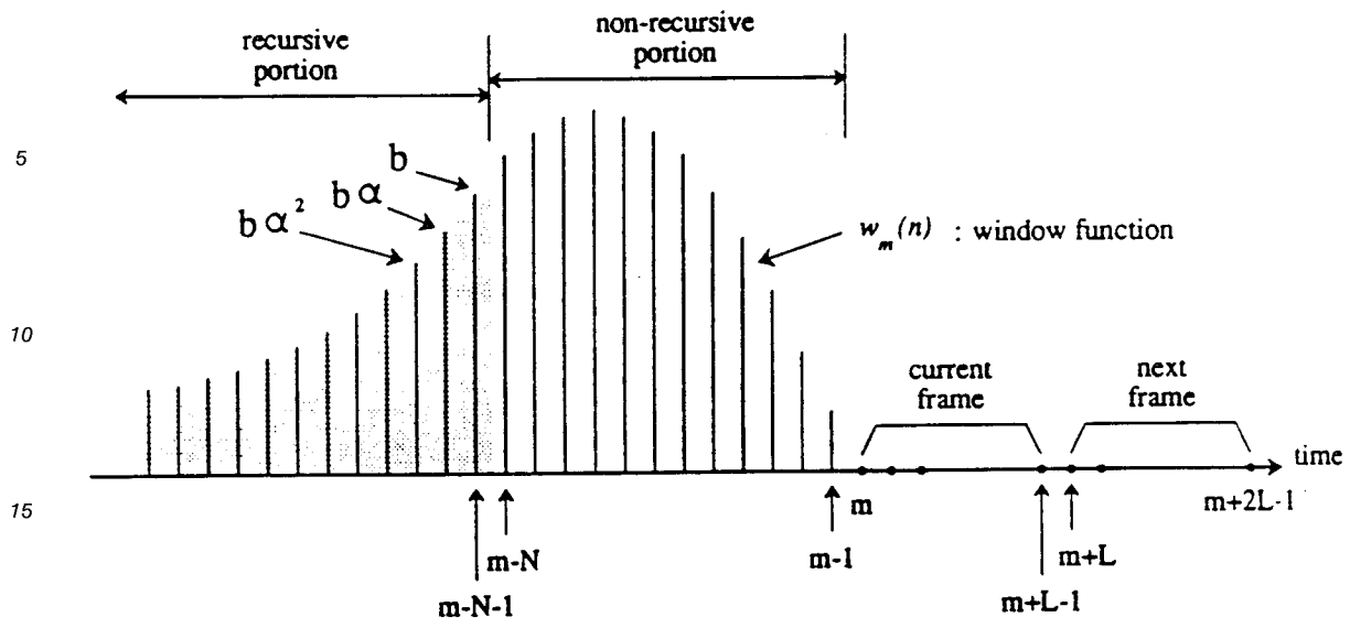
Figure 4(b)/G.728 Illustration of a hybrid window
