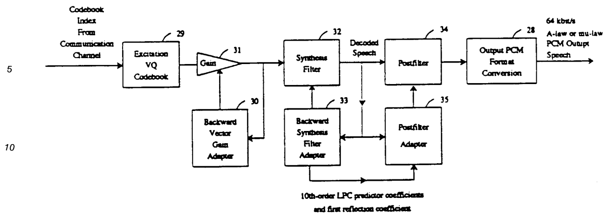
Figure 3/G.728 LD-CELP Decoder Block Schematic
