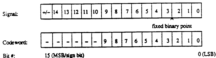
FIGURE I-5/G.728
