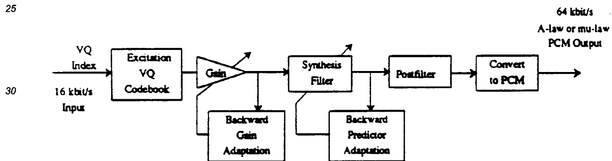
LD-CELP Decoder
