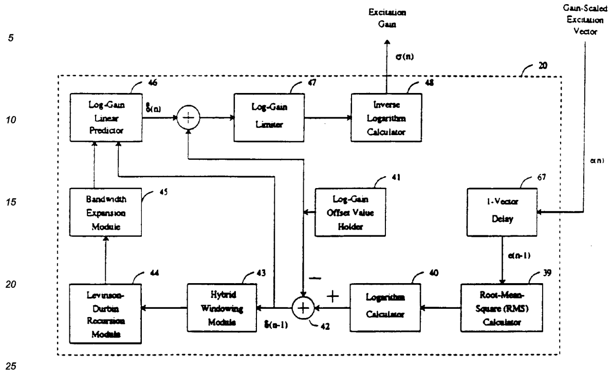
Figure 6/G.728 Backward Vector Gain Adapter
