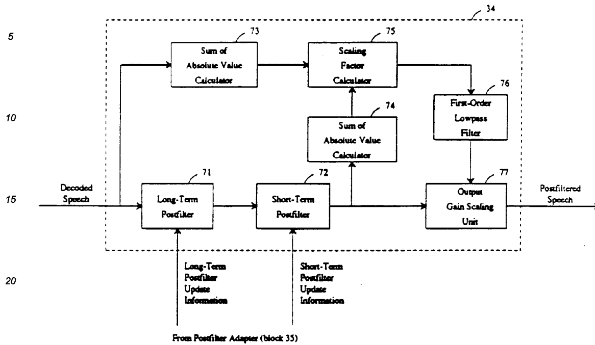
Figure 7/G.728 Postfilter Block Schematic
