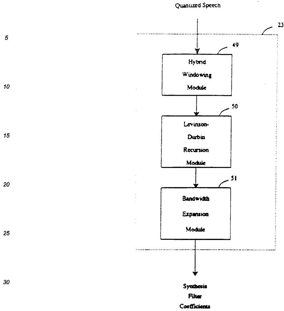
Figure 5/G.728 Backward Synthesis Filter Adapter
