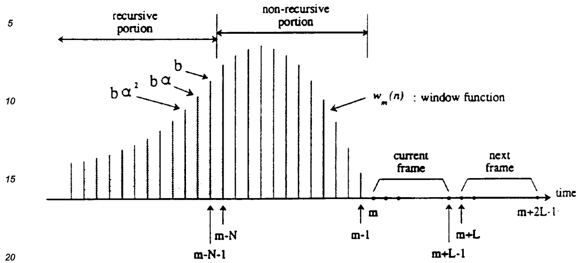
Figure 4(b)/G.728 Illustration of a hybrid window
