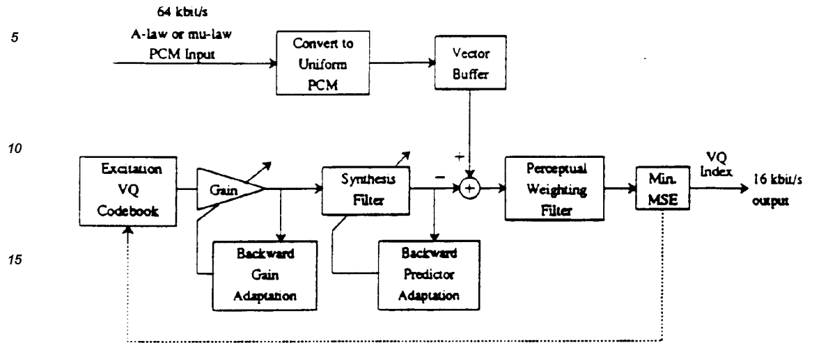
LD-CELP Encoder
