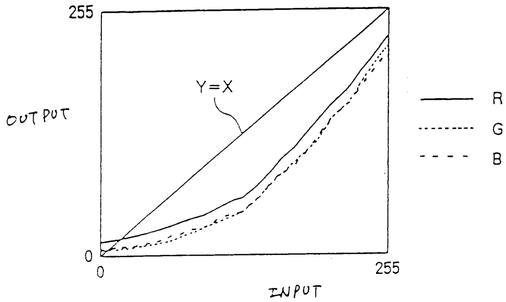
PRINTER CALIBRATION \gamma CURVE
