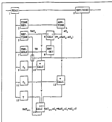
FIG. 1 Hardware Implementation using Arrival Times
