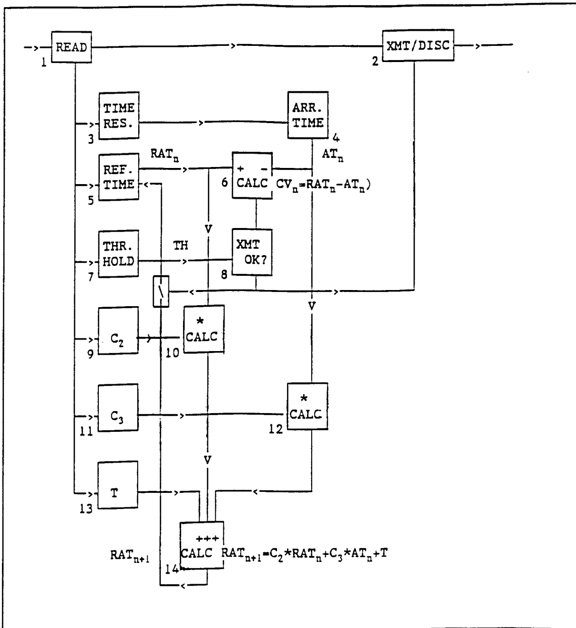
FIG. 1 Hardware Implementation using Arrival Times
