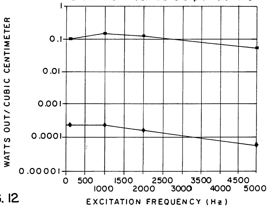
FIG. 12 ROTARY TRANSFORMER OUTPUT PER CC VS. FREQUENCY EXCITATION VOLTAGE IS 5Vp OR 3.5VRMS
