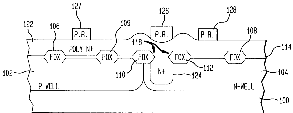
FIG. 2D
