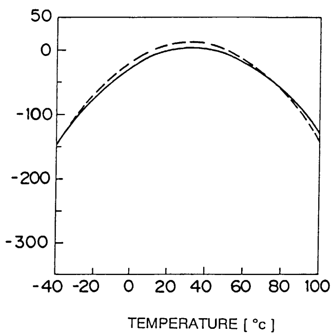
FIG. 5 TEMPERATURE CHARACTERISTIC OF CENTER FREQUENCY [ ppm/°c ]
