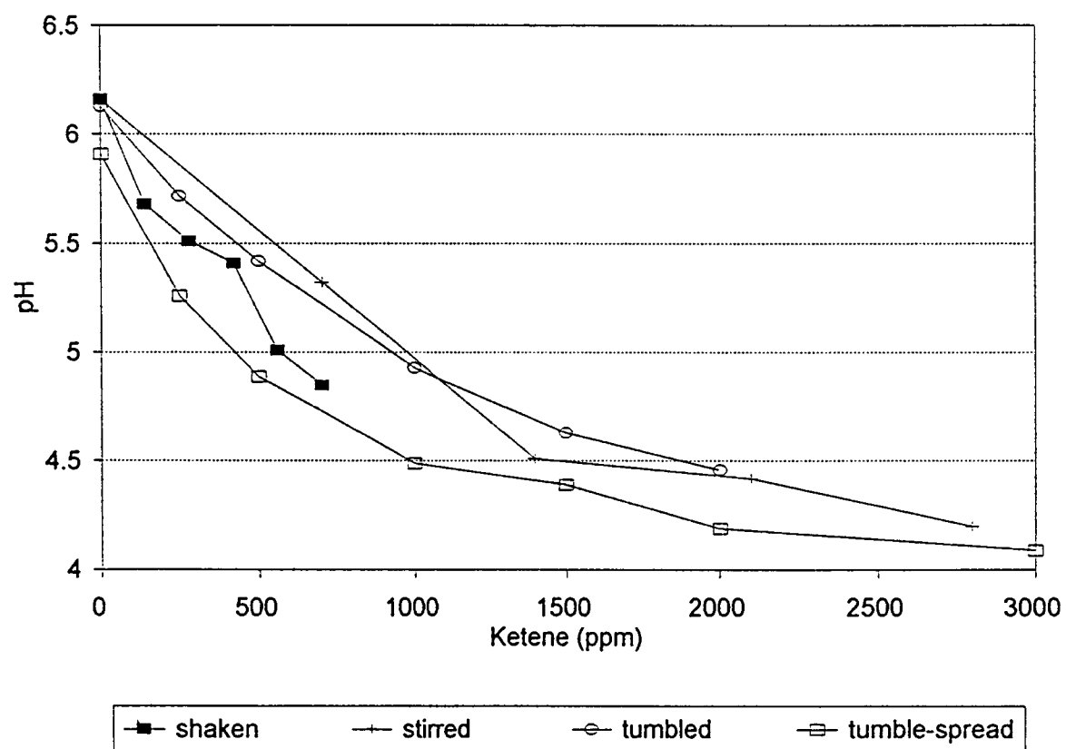
Figure 4. pH of ketene-treated flour
