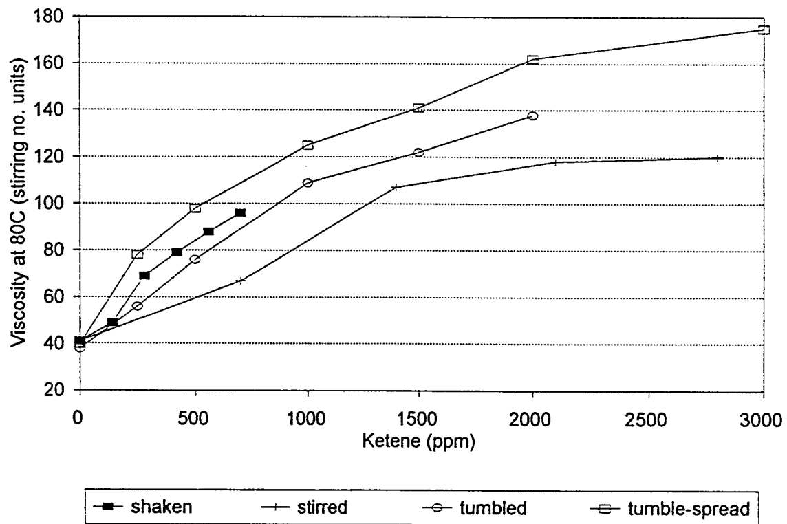
Figure 3. RVA properties of ketene-treated flour.
