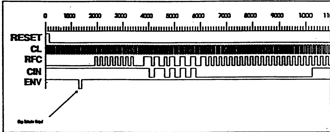
Waveforms with gap detection and synchronization
