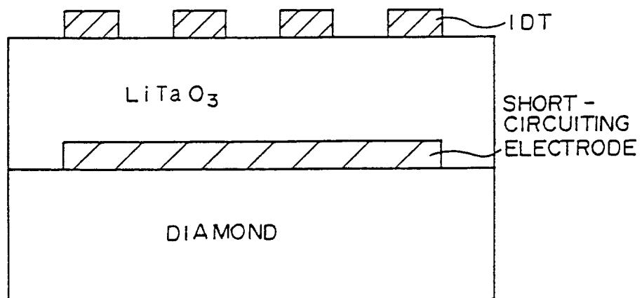
( ELECTRODE ARRANGEMENT F )
