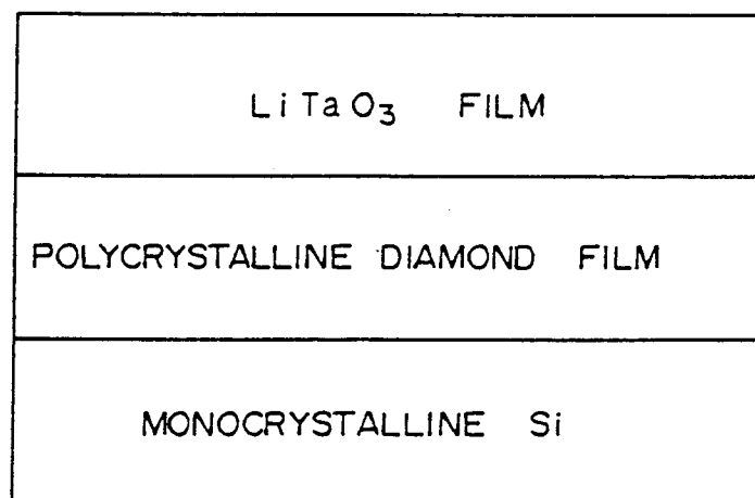
( LAYER STRUCTURE 2 )
