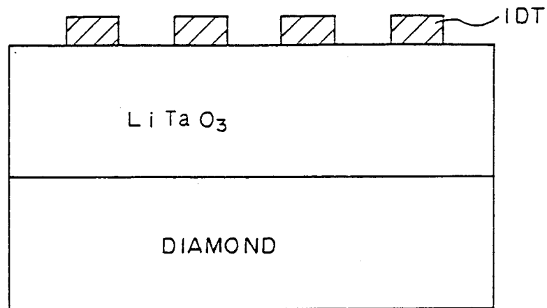
( ELECTRODE ARRANGEMENT E )
