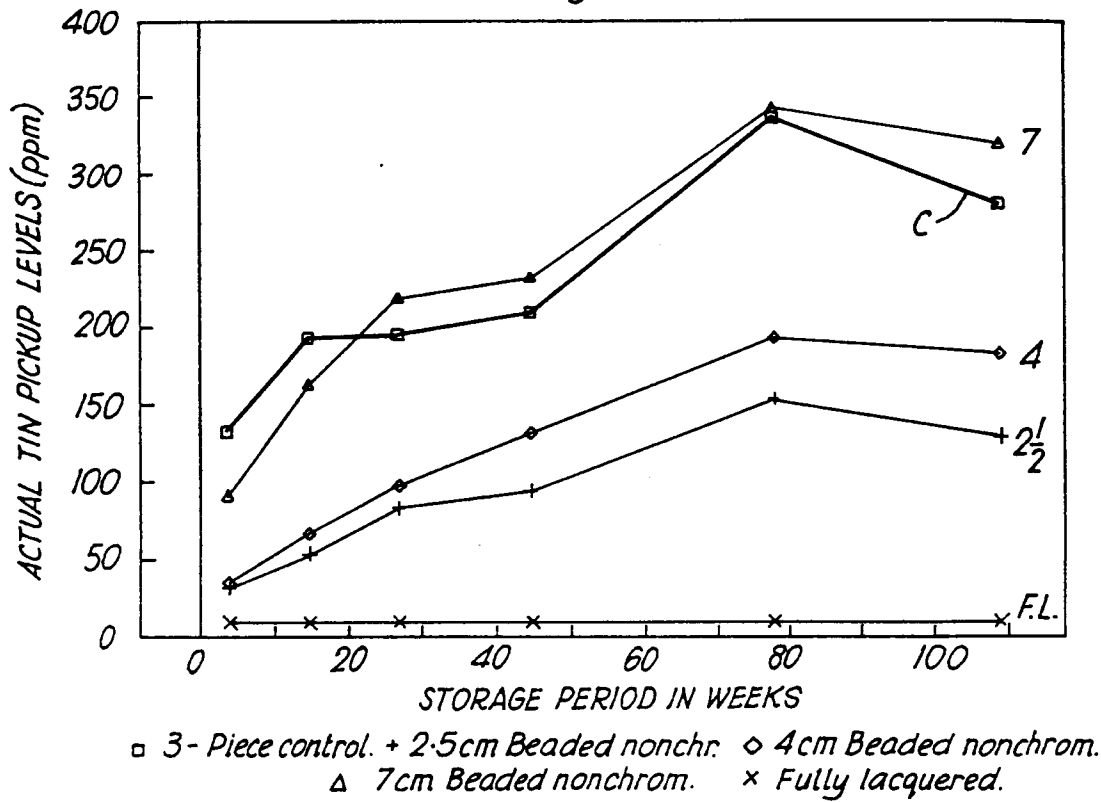
Fig. 8b. PASTA IN TOMATO SAUCE - AMBIENT. T2BA, 35M, 13.8g/m 2 , ET + LAC. ENDS.
