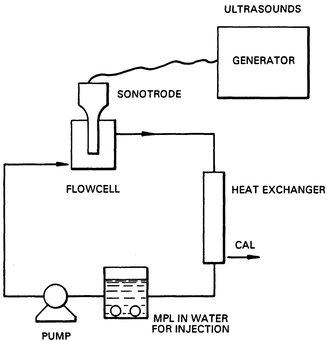
SONICATION LOOP
