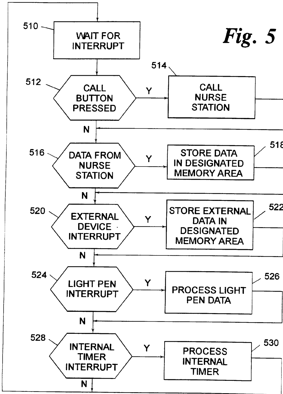
PATIENT STATION MAIN LOOP
