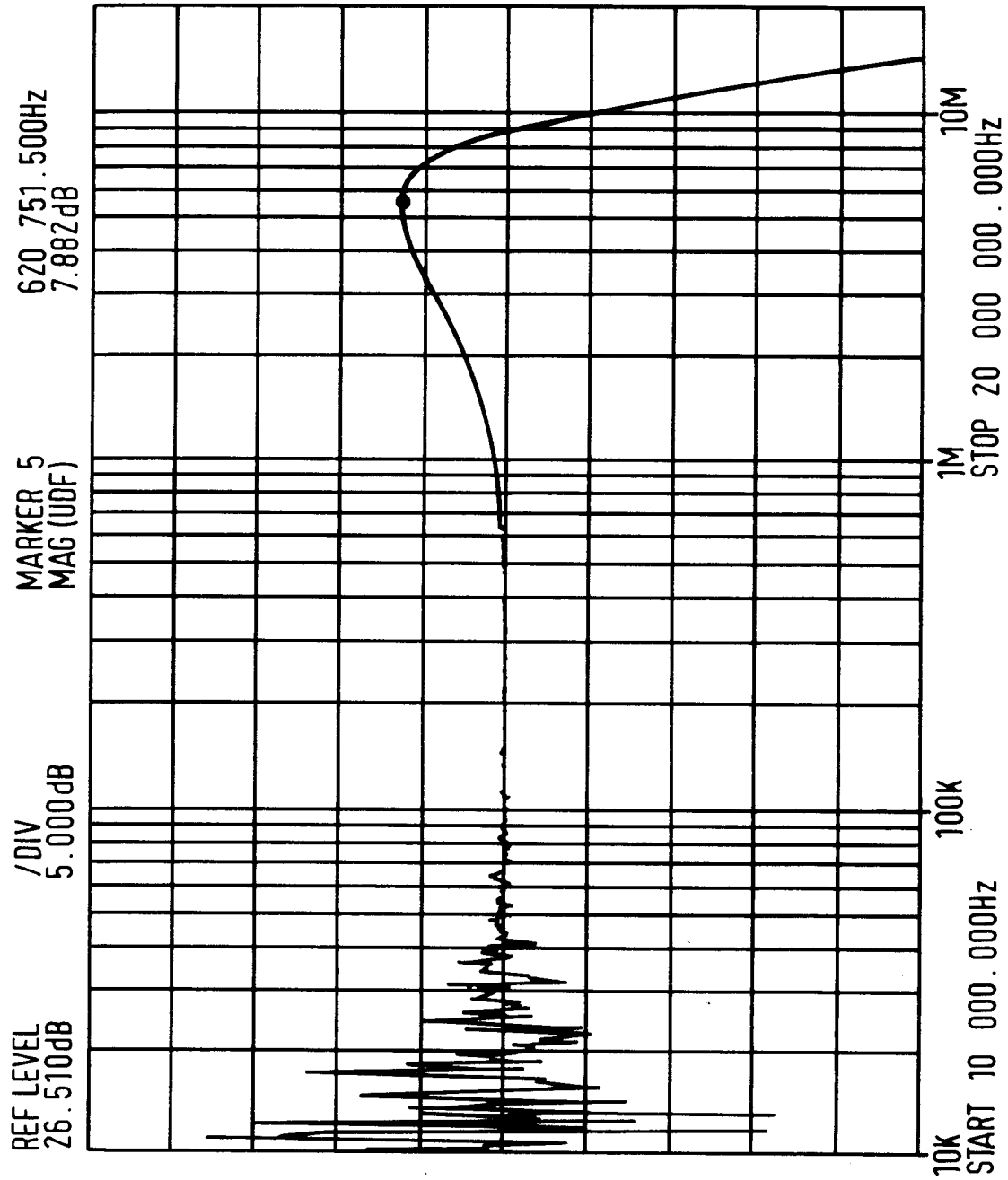
FIG. 14B EQUALIZER
