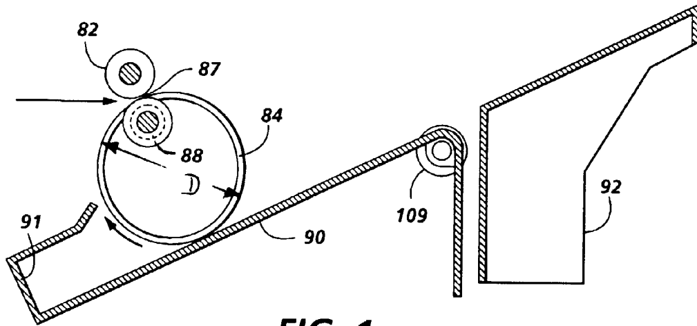
FIG. 1 PRIOR ART
