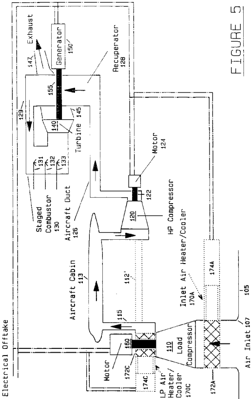
ALTERNATIVE CONFIGURATION 1
