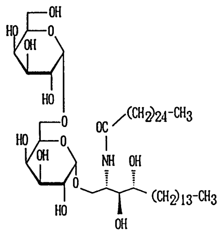
COMPOUND 33
