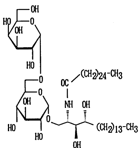
COMPOUND 31
