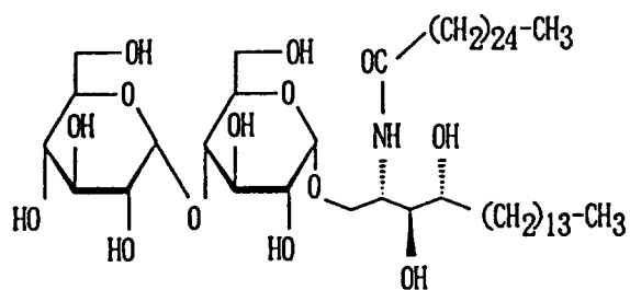
COMPOUND 35
