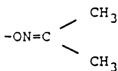
Acetone Oxime
