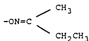
Methylethyl Ketoxime
