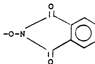
Oxyphthalimide
