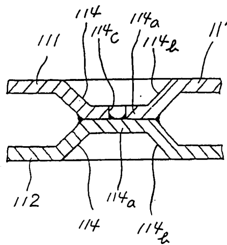
Fig. 3 (Prior Art)
