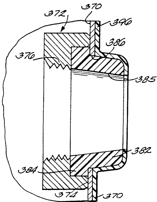
Fig. 13C PRIOR ART
