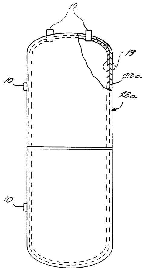
Fig. 17 PRIOR ART
