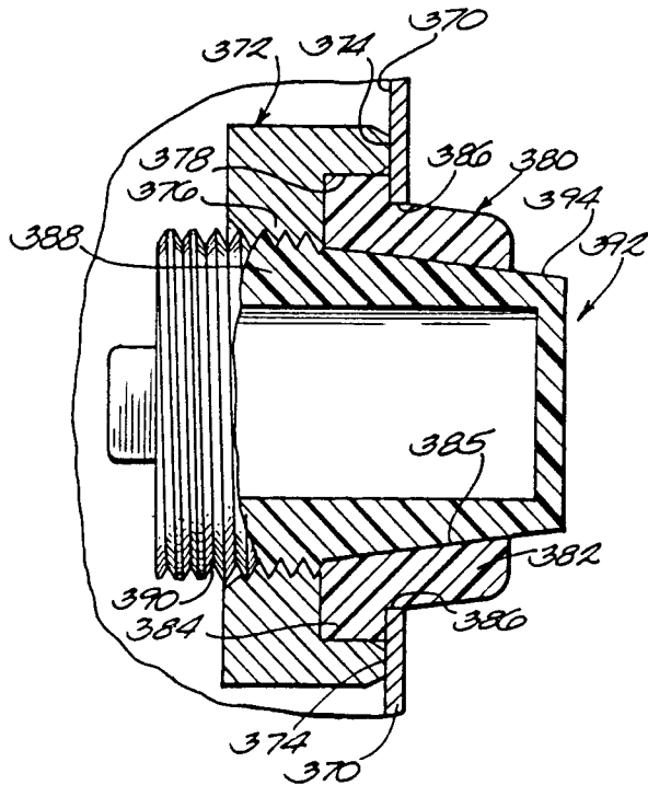
Fig. 13A PRIOR ART
