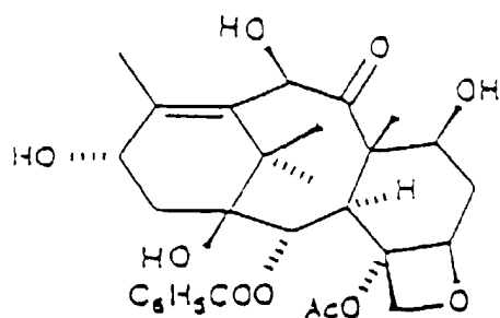
10-DESACETYLBACCATINE III
