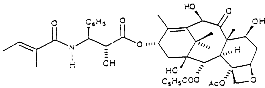
10-DESACETYLCEPHALOMANNINE
