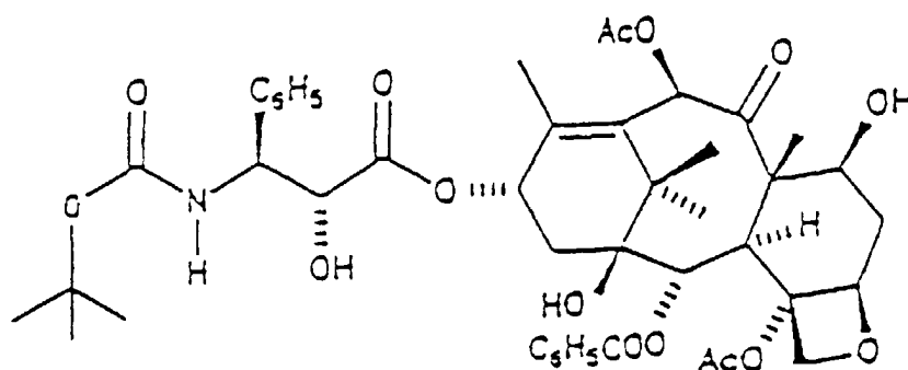
DOCETAXAL
