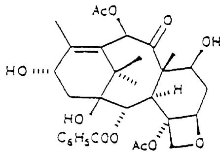
BACCATINE III
