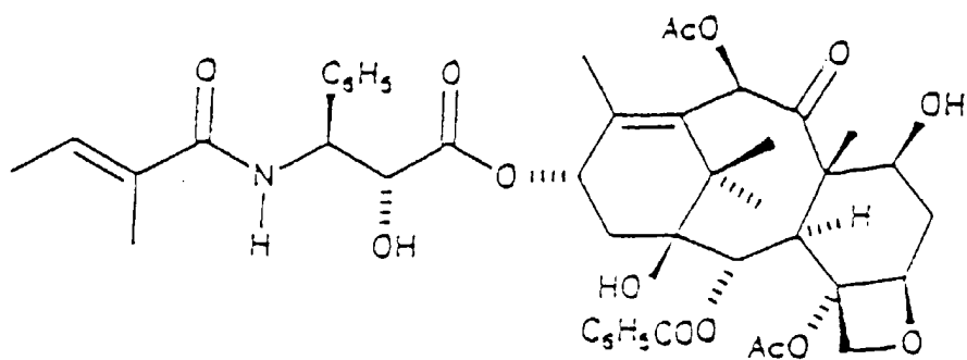
CEPHALOMANNINE
