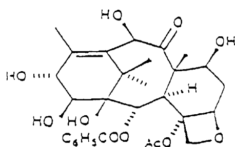
14β-HYDROXY-10-DESACETYLBACCATINE III
