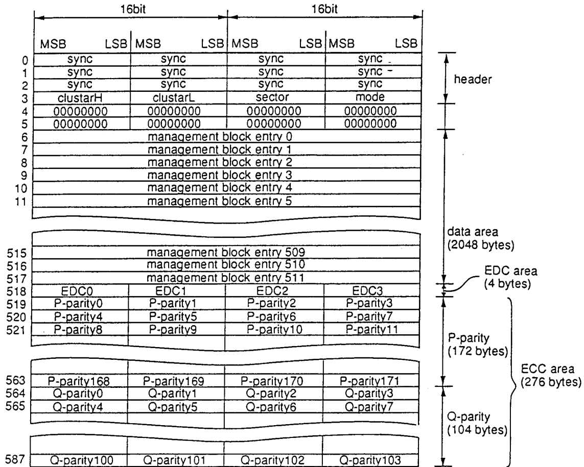
Center structure of management table
