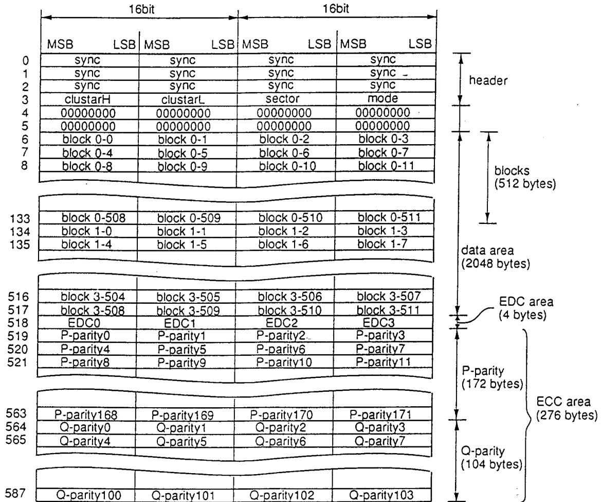
boot area sector structure (1)
