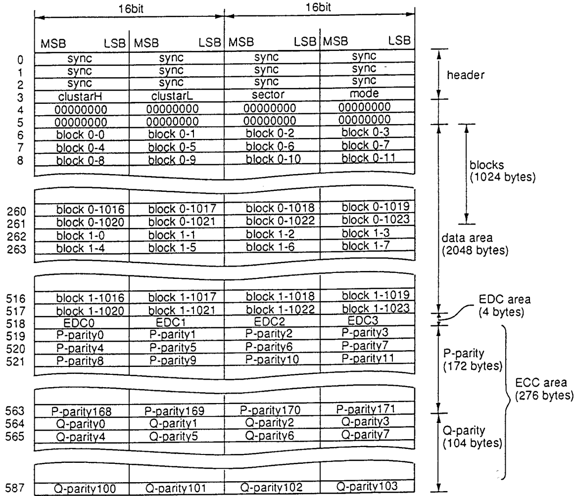
boot area sector structure (2)
