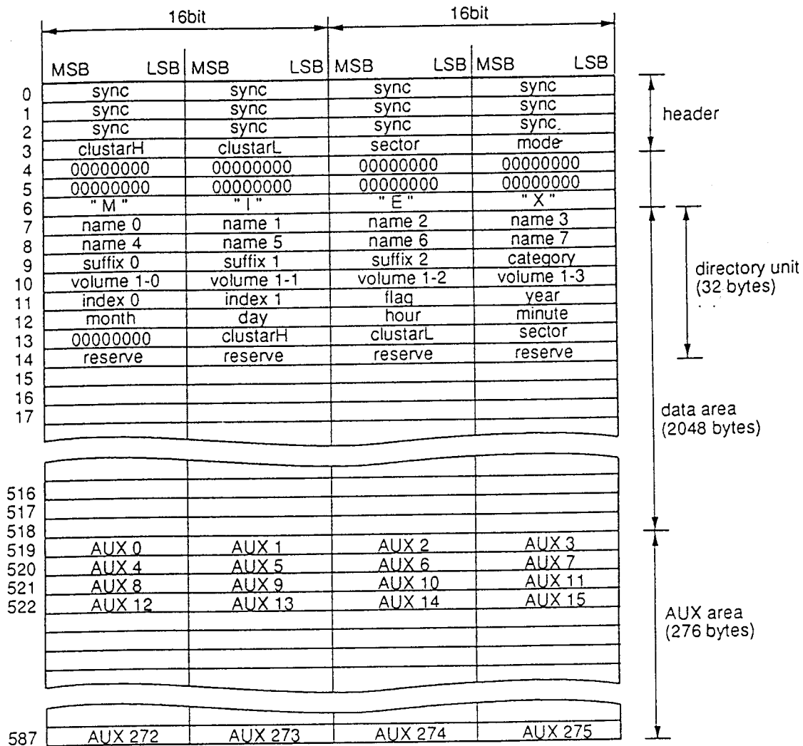
simple U-TOC sector structure (directory sector)
