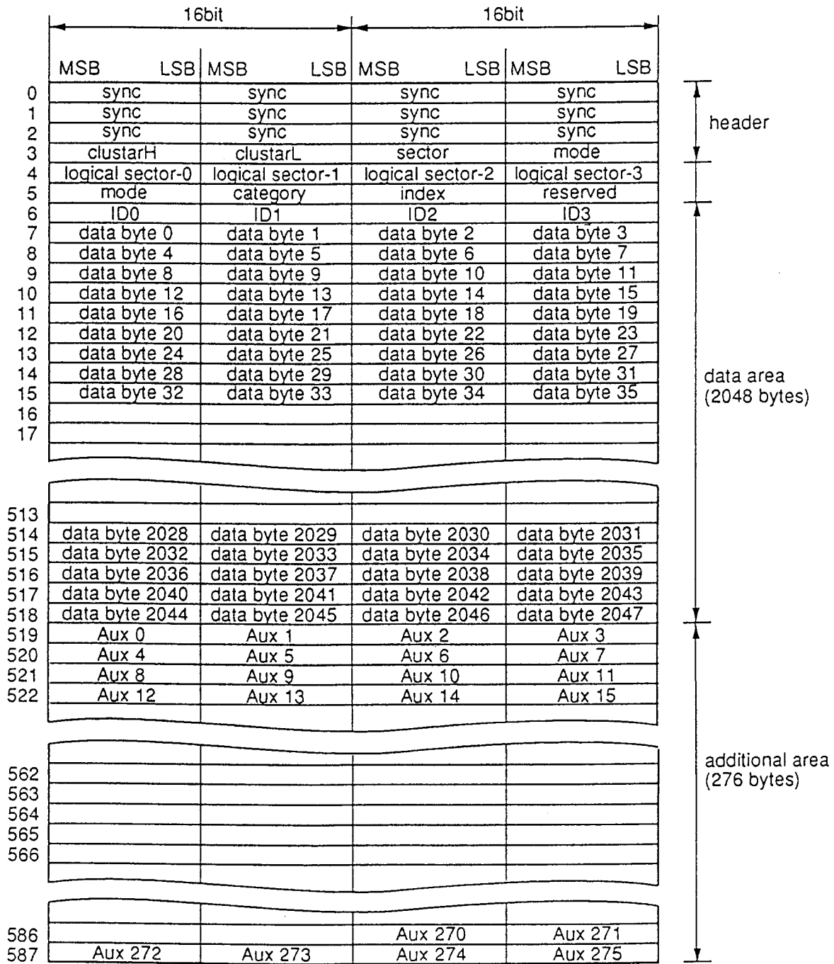
data sector structure
