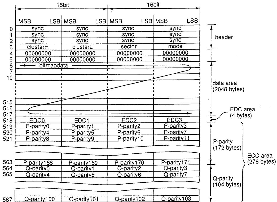
Volume space bitmap sector structure
