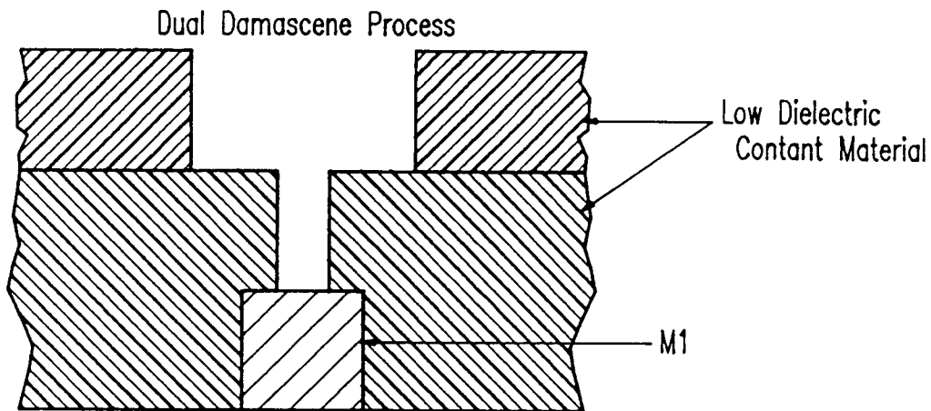
FIG.9A Formation of a Via/Line
