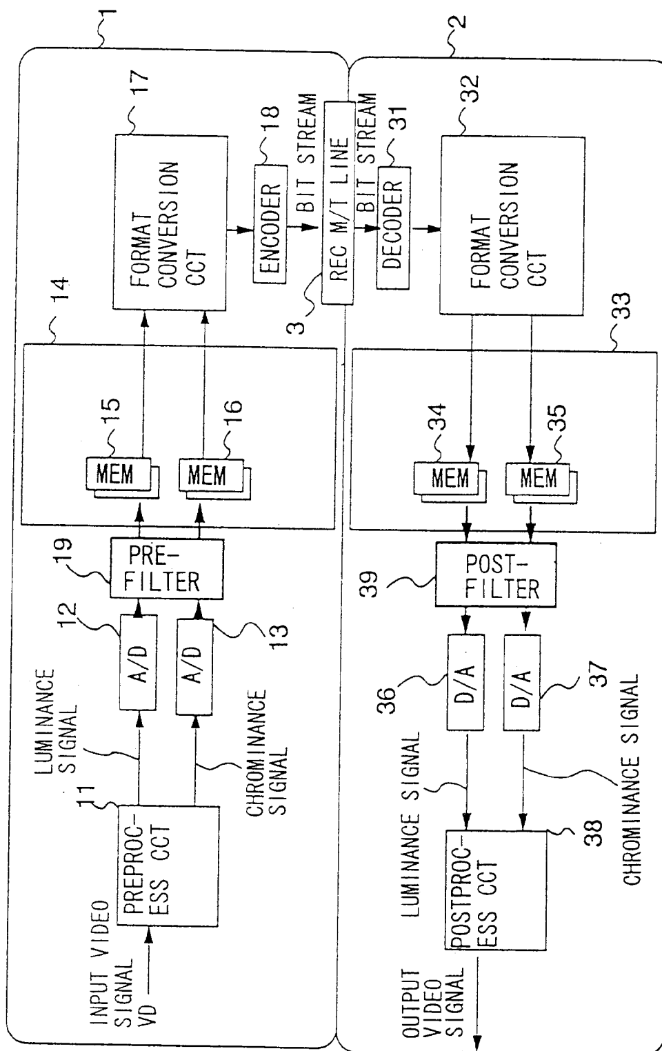
FIG. 4 (RELATED ART)
