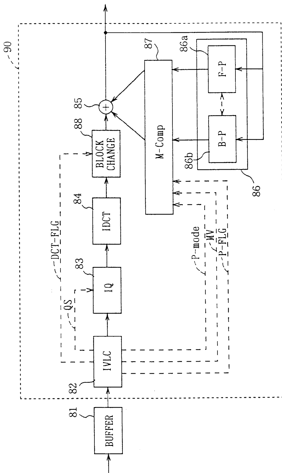
FIG. 9 (RELATED ART)
