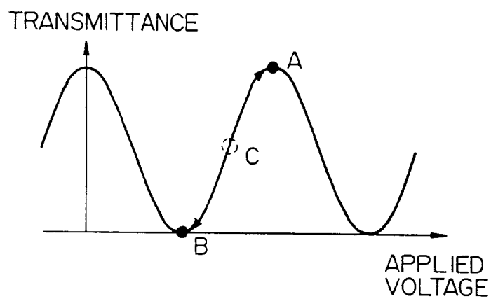
Fig. 14 PRIOR ART
