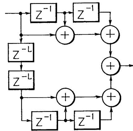
TWO-DIMENSIONAL FILTER (LPF)
