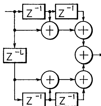
TWO-DIMENSIONAL FILTER (LPF) FIG. 42B
