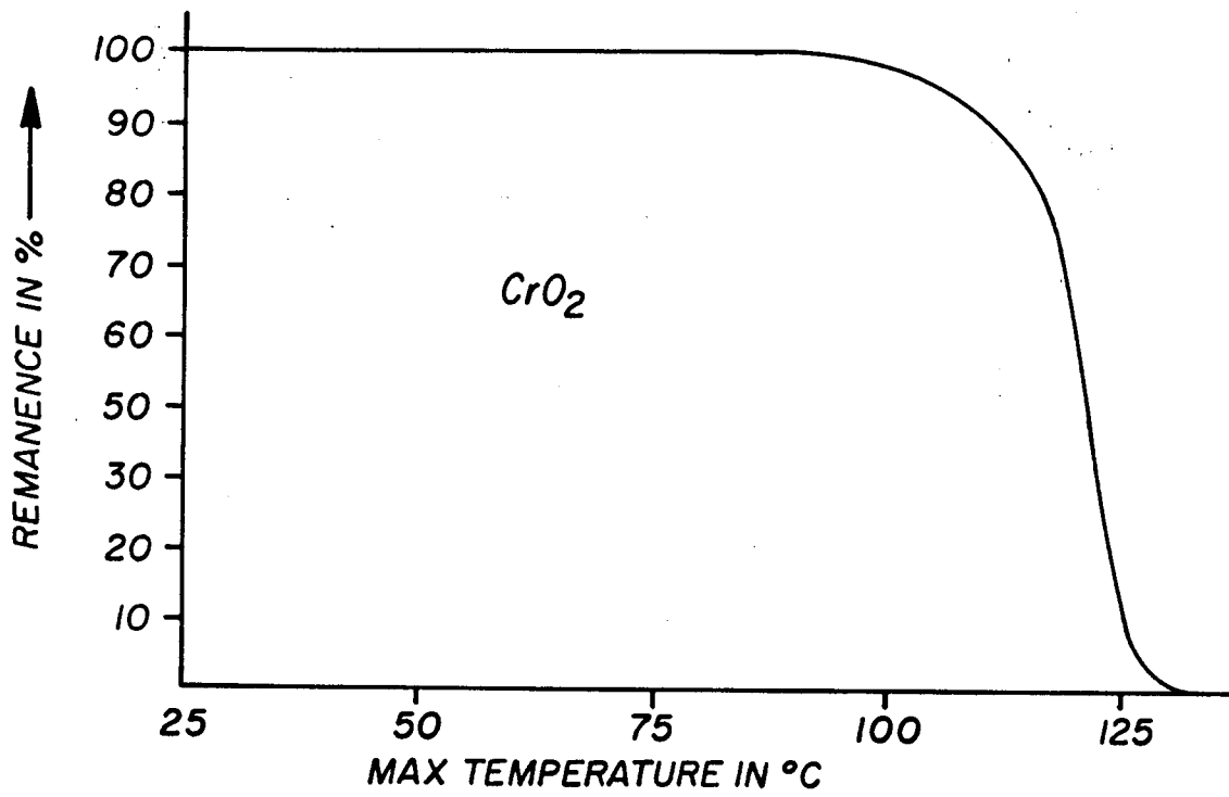
FIG. 1 (PRIOR ART)
