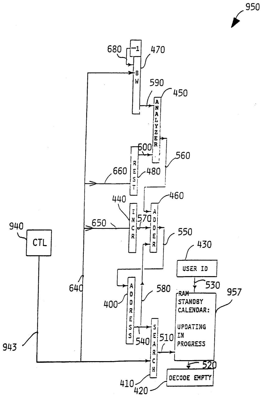
FIG. 10 PLACEMENT DEVICE
