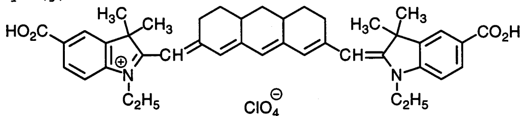
Dye (j)
