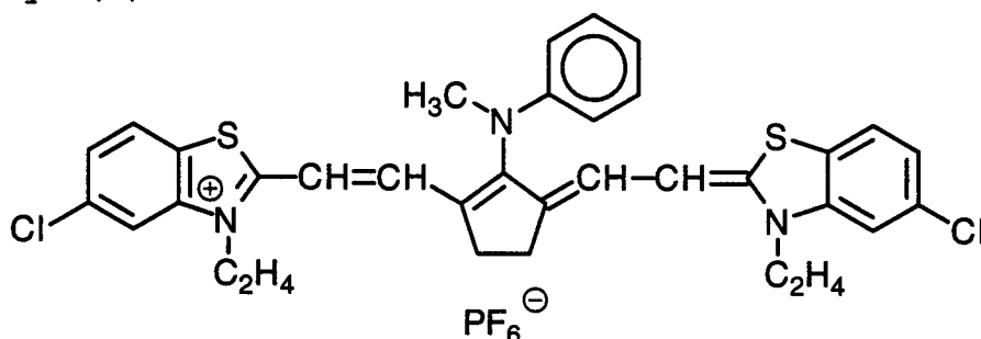
Dye (f)
