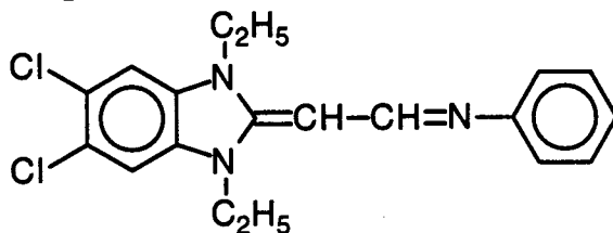
Compound C
