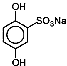
Compound B
