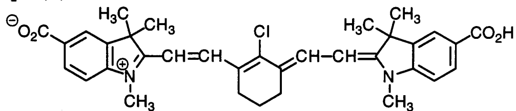
Dye (b)
