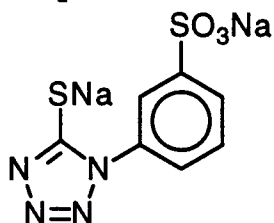
Compound F
