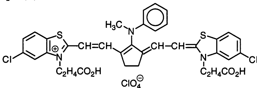
Dye (c)
