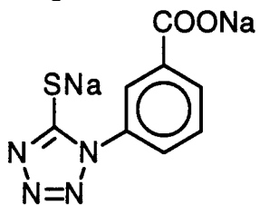
Compound D
