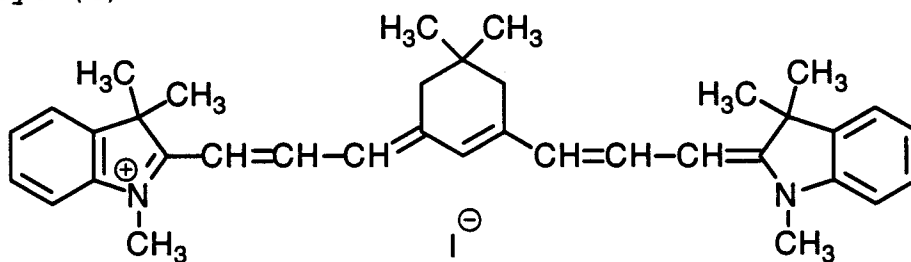
Dye (i)
