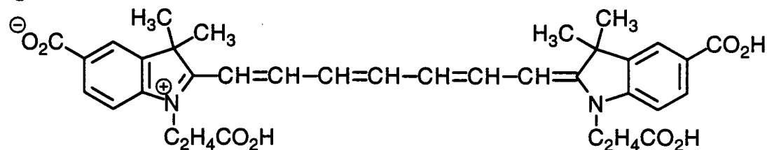
Dye (e)
