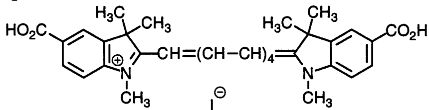
Dye (h)
