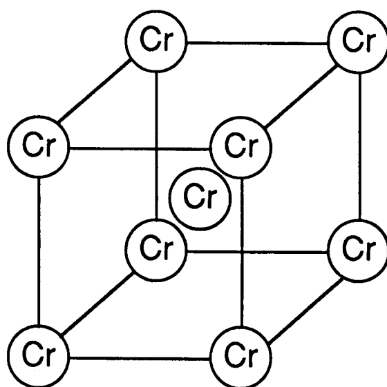
Cr, BCC a = .2884
