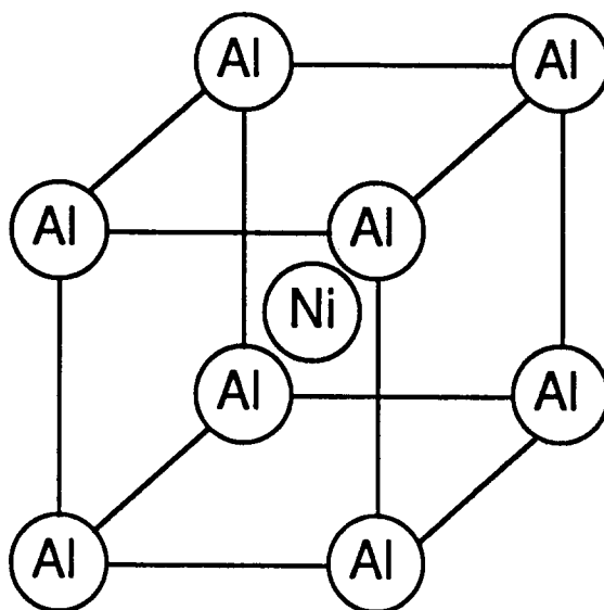
NiAl, B2 a = .2887
