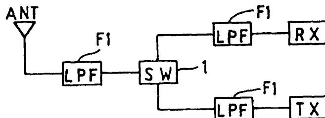
FIG.10 PRIOR ART
