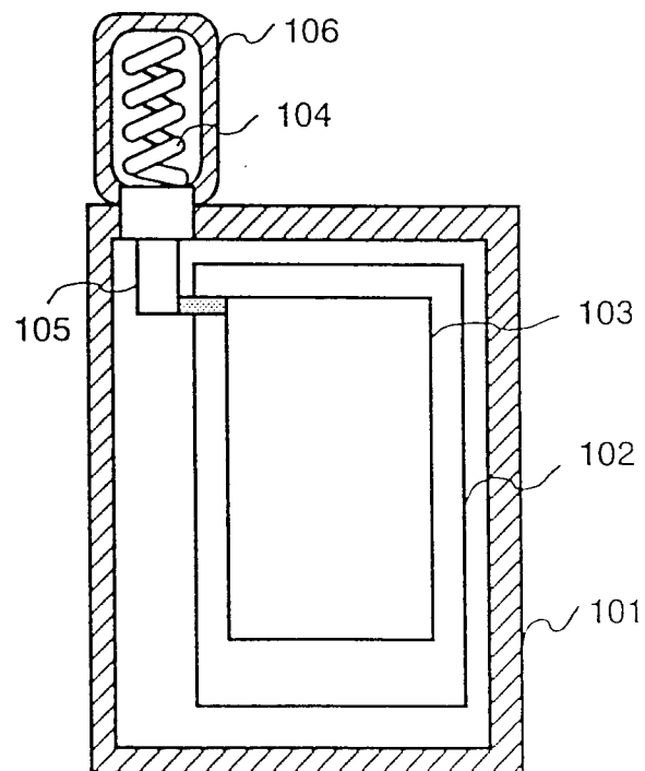
Fig.14 CONVENTIONAL ART
