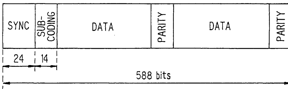
FRAME STRUCTURE
