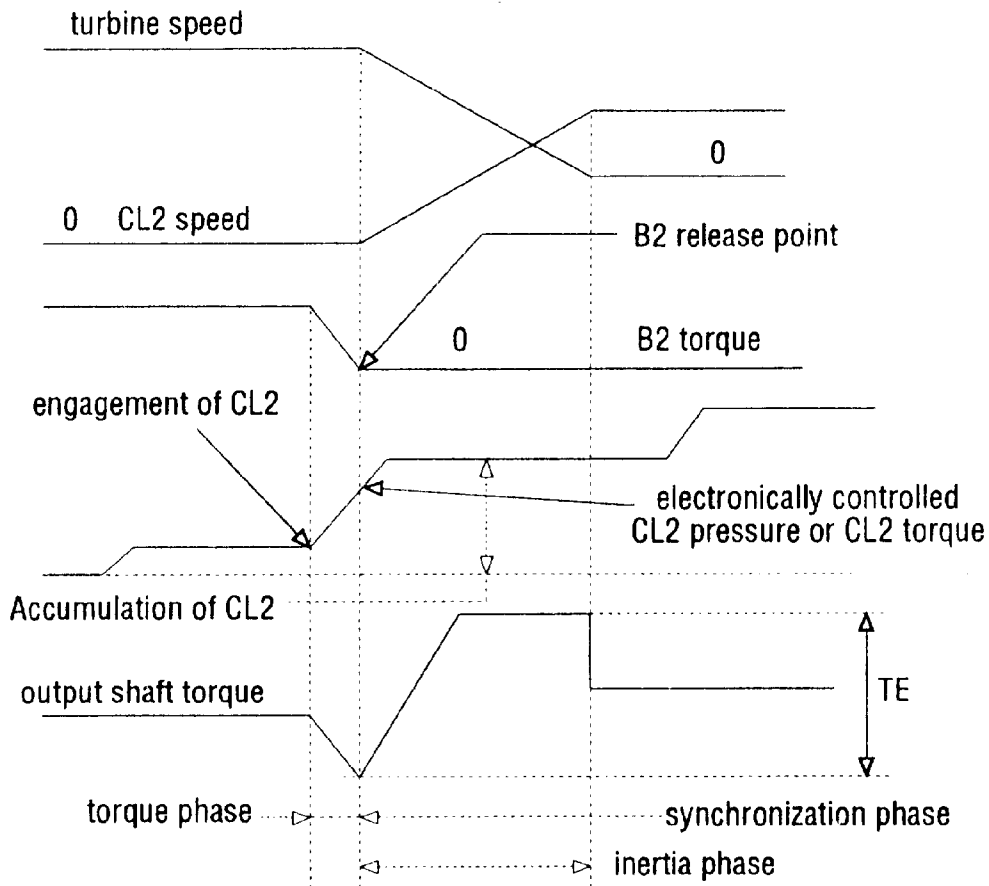
Fig. 6 (2-3 UPSHIFT)
