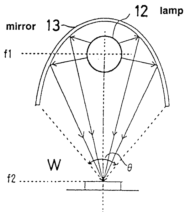
Schematic of an arrangement of a lamp, a mirror and a workpiece for the light irradiator
