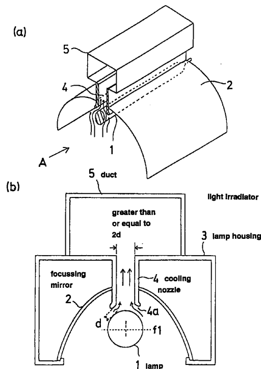
Schematic of the first embodiment of the invention
