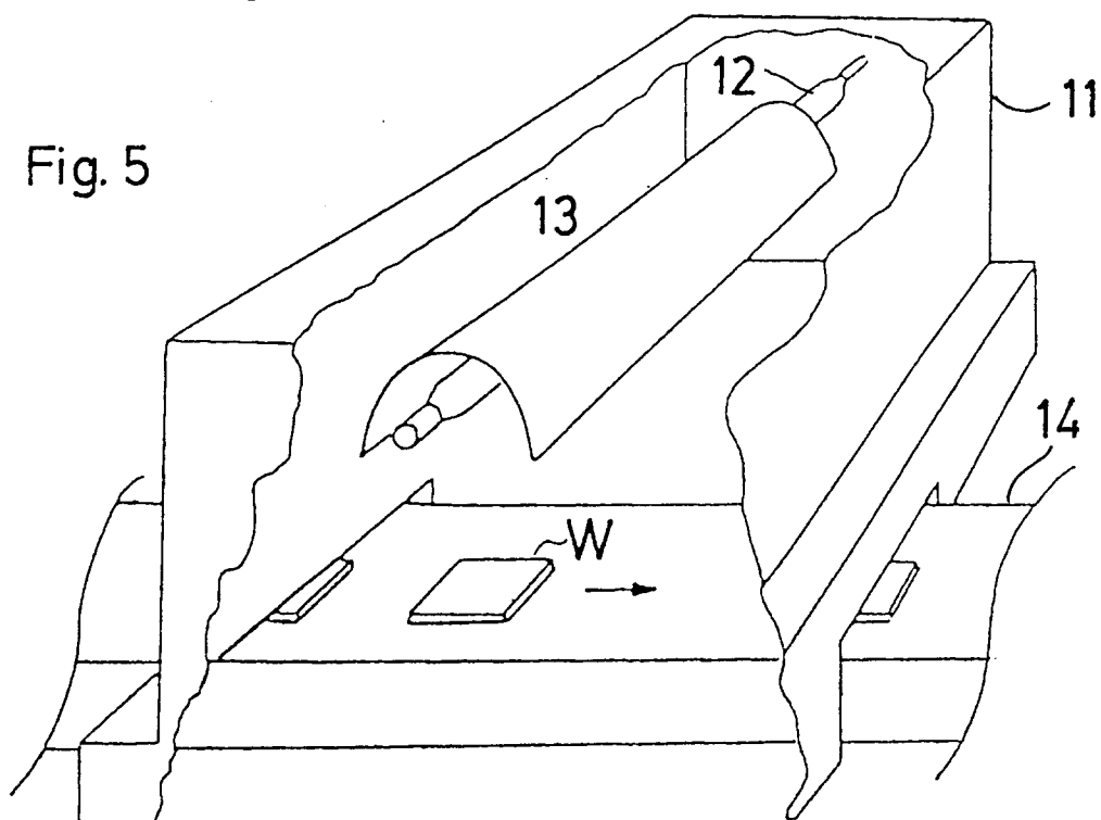
Schematic of one example of a treatment device using a light irradiator
