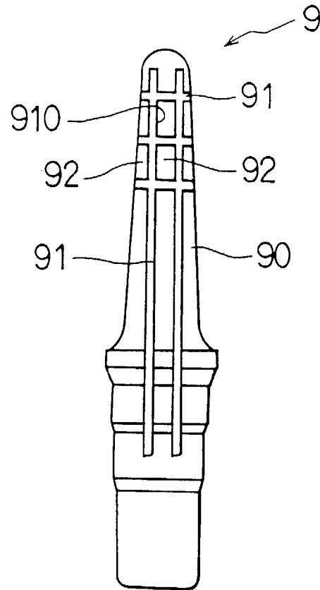
FIG. 9 PRIOR ART
