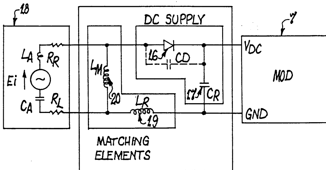
SERIES RESONANT CIRCUIT
