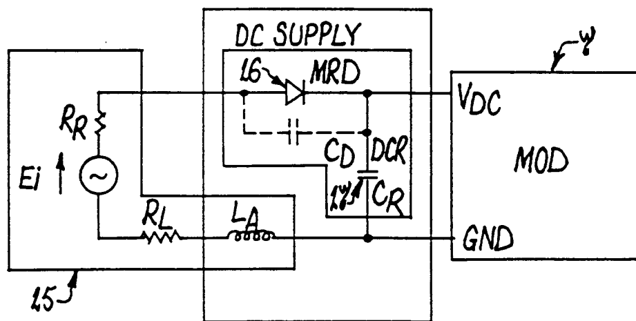
SERIES RESONANT CIRCUIT
