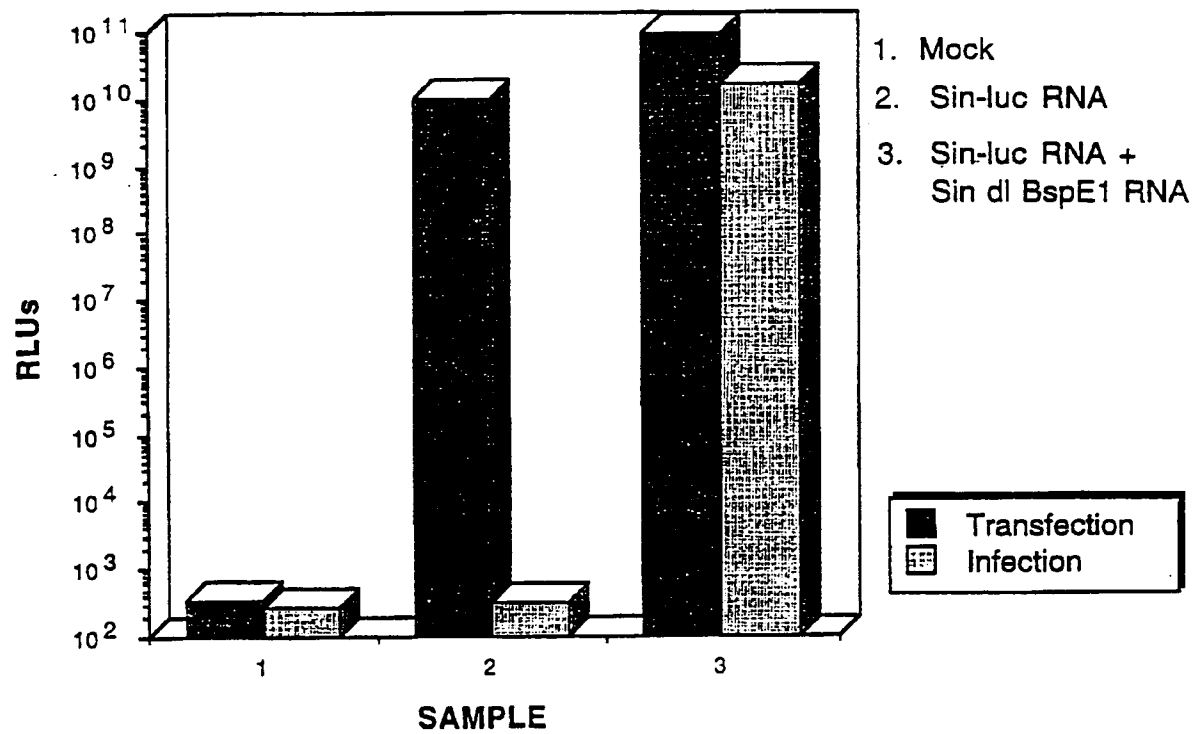
Figure 6: Expression and Rescue of the Sindbis-luciferase Vector
