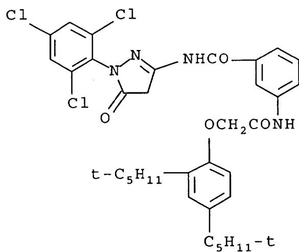
Coupler M-1
