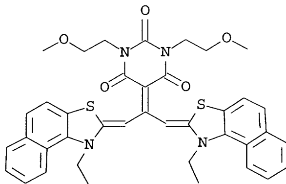
Red Sensitizing Dye-3
