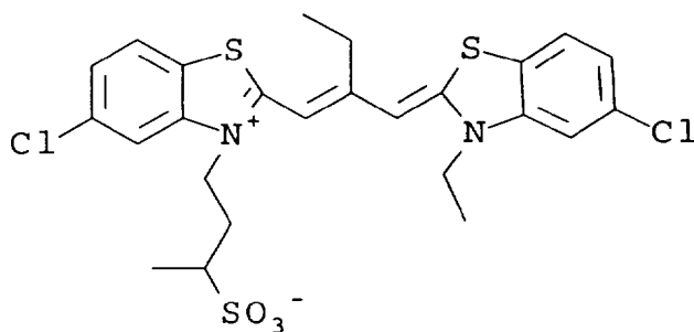
Red Sensitizing Dye-1
