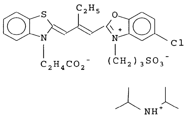
Green Sensitizing Dye-3
