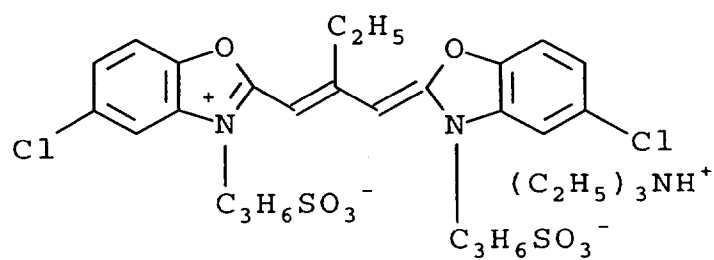
Green Sensitizing Dye-2
