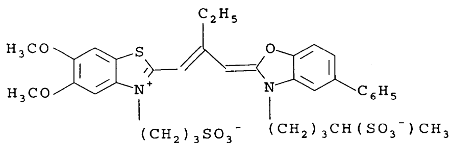
Red Sensitizing Dye-1
