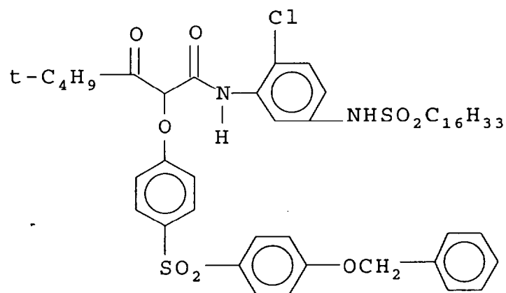
Coupler Y-2
