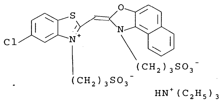
Blue Sensitizing Dye-1
