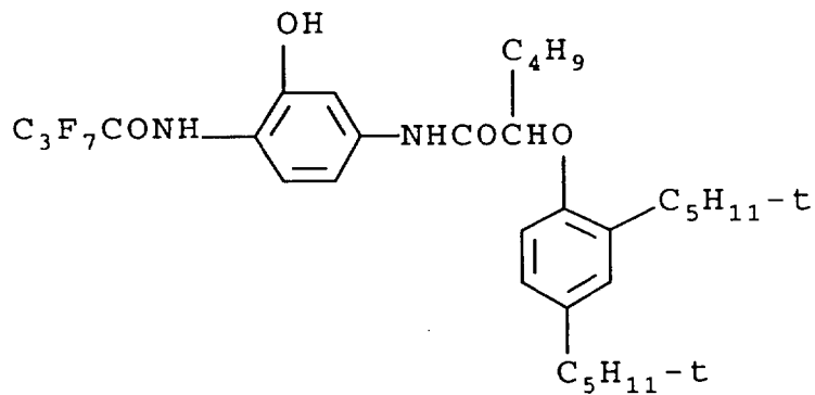
Coupler C-1
