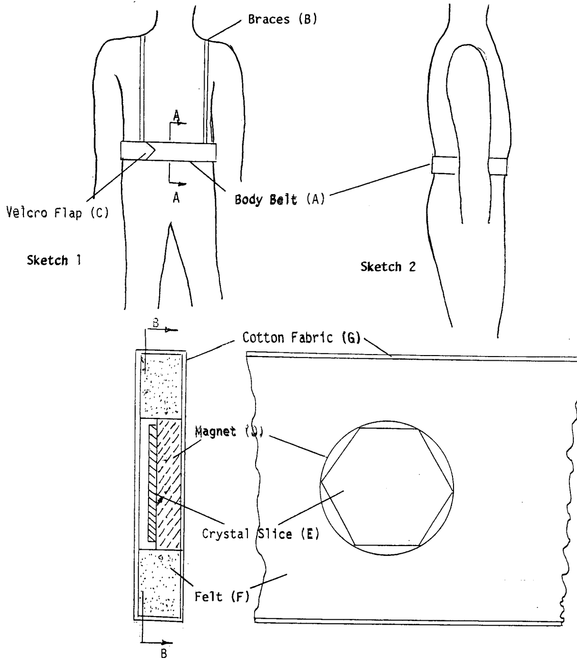
Section A - A (Scale - Full Size) Section B - B (Scale - Full Size)
