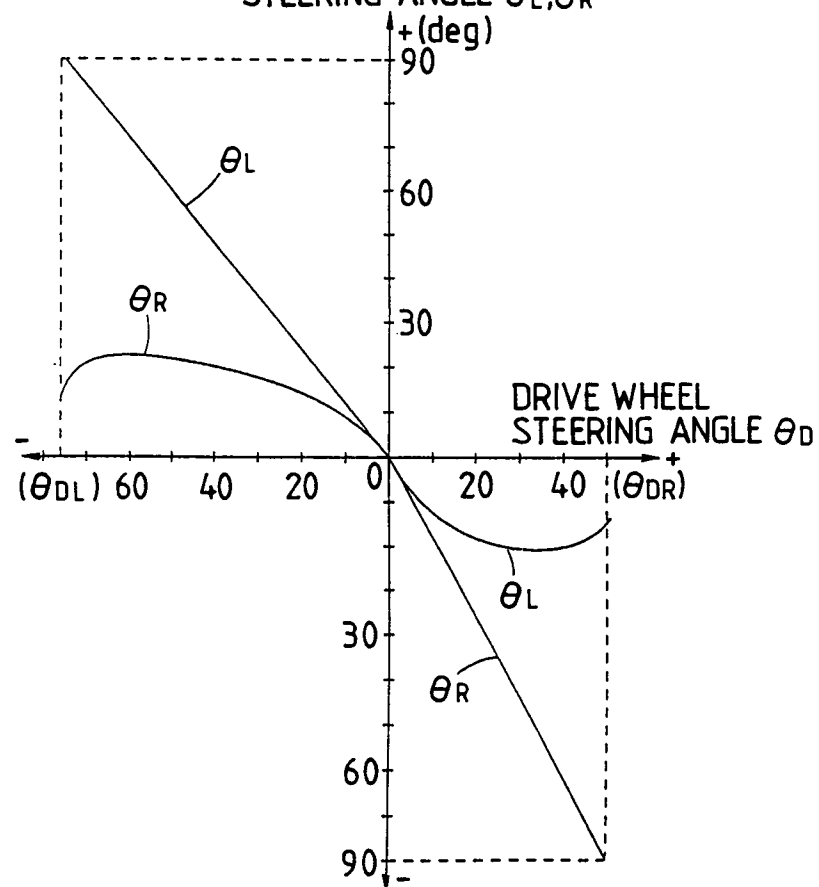
FIG. 33 LOAD WHEEL TARGET STEERING ANGLE \theta_L, \theta_R
