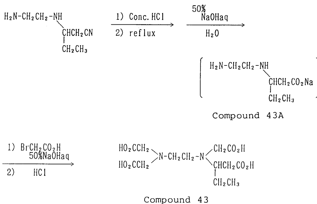
Scheme 6
