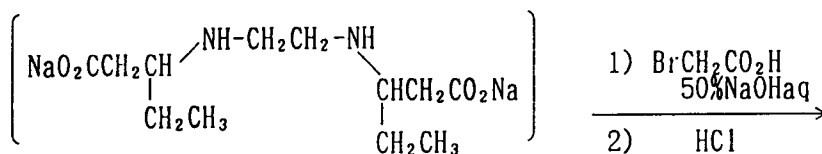
Compound 42A
