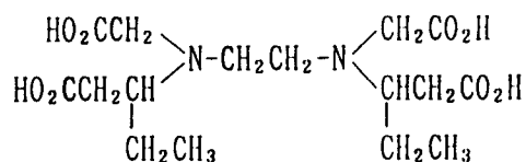
Compound 42
