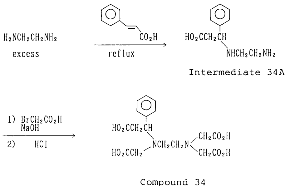
Scheme 8
