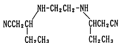
Intermediate 42C
