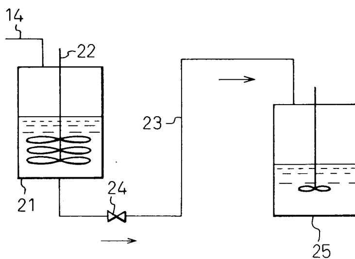
Fig.3 PRIOR ART
