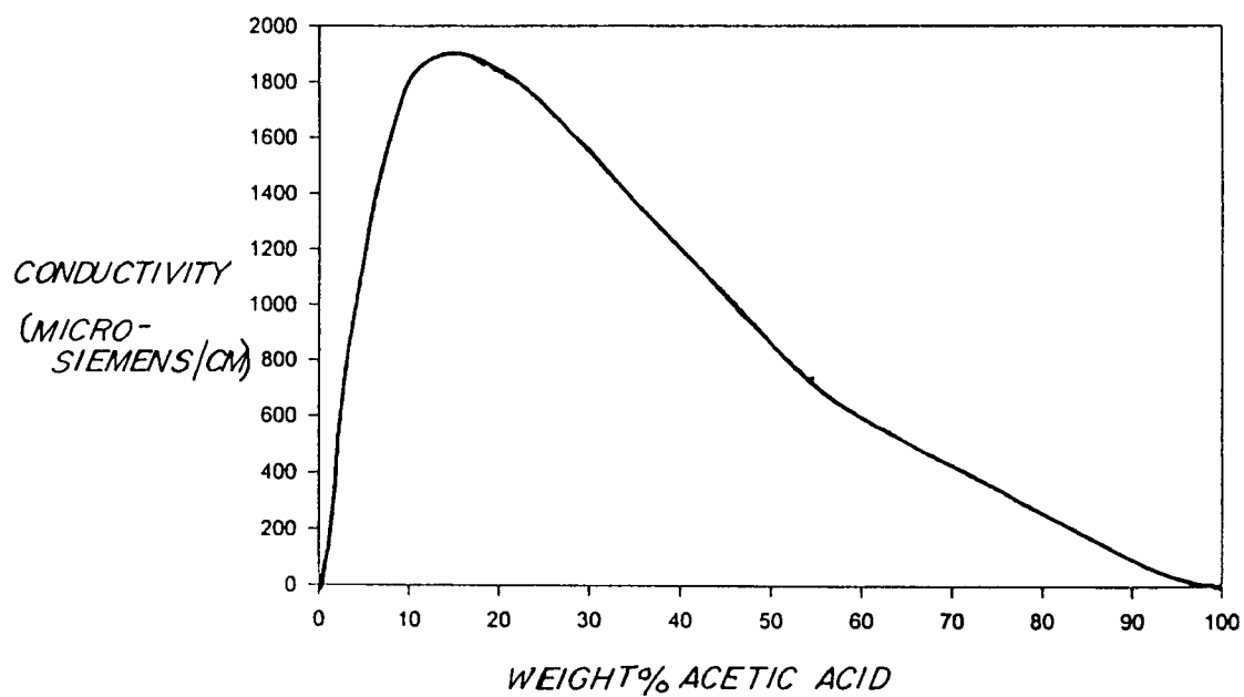
Acetic Acid Conductivity Curve @ 25 C
