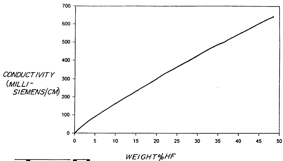
Hydrofluoric Acid Conductivity Curve @ 25 C
