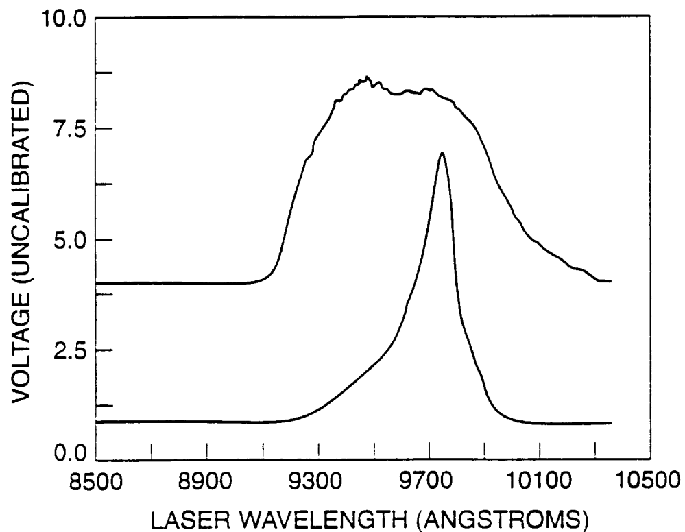
EXCITATION SCAN OF REPORTER ALONE: LIF COLLECTED AT 5410 Å
