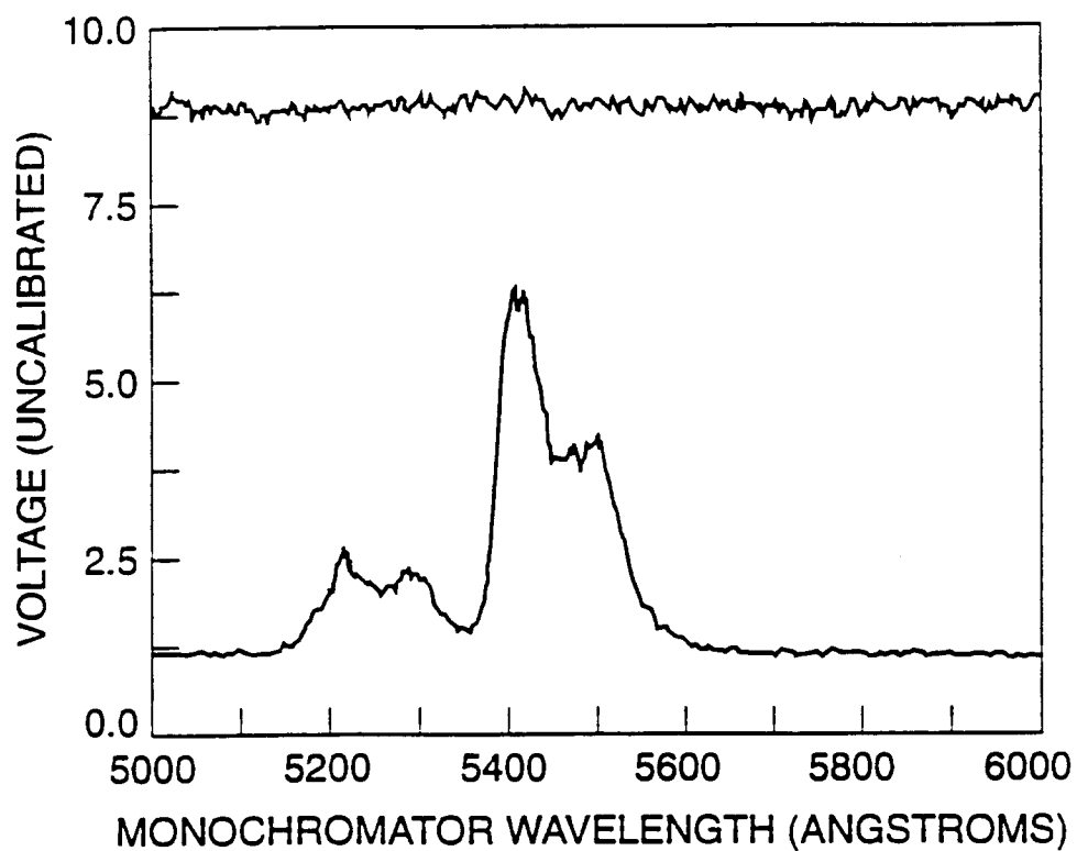
FLOURESCENCE SCAN OF REPORTER ALONE: EXCITATION AT 9772
